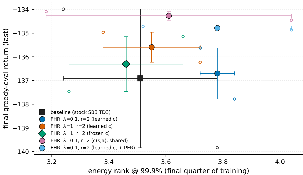
Pendulum-v1 - penalised-window compression vs return
