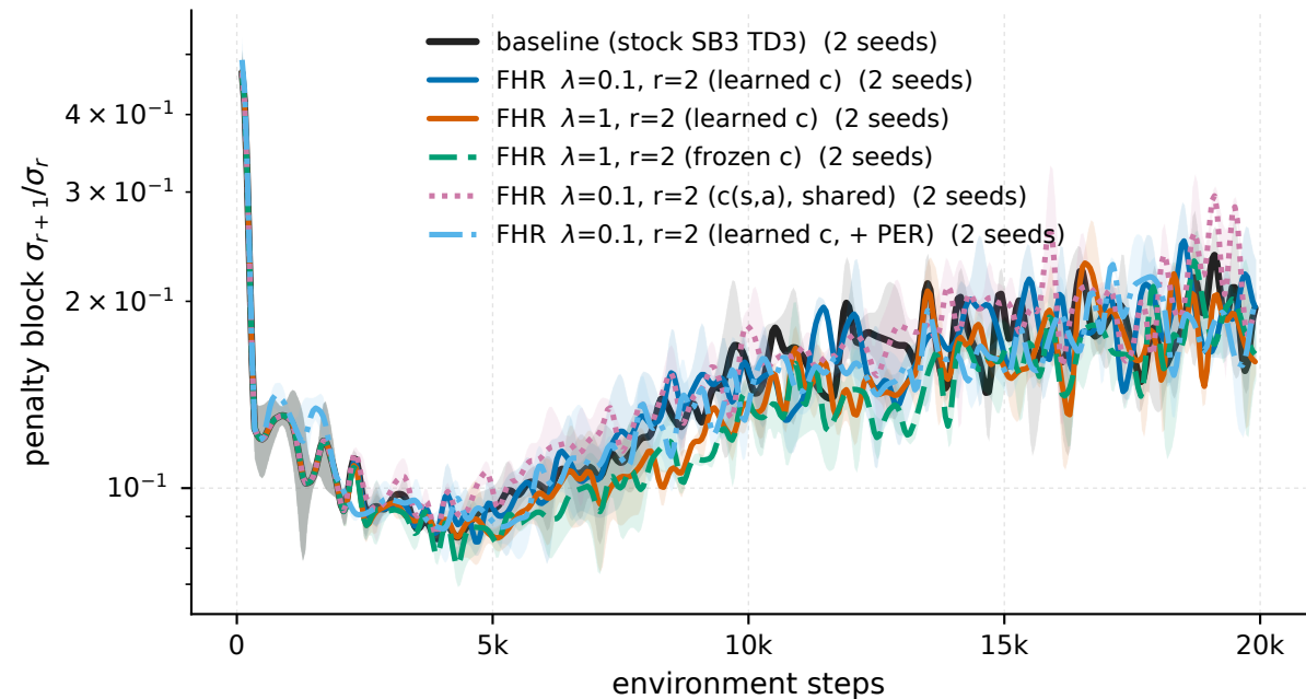
Pendulum-v1 - penalised windows: \sigma_{r+1}/\sigma_r of the penalty block
