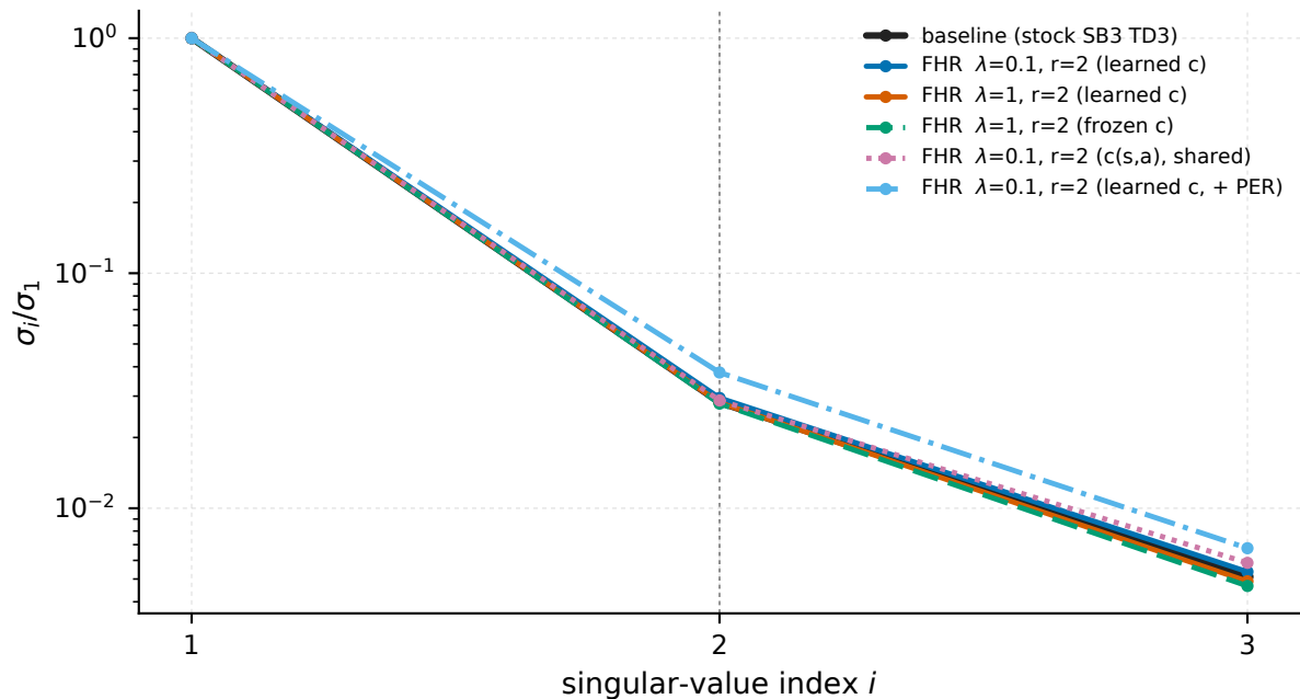
Pendulum-v1 - penalty block spectrum, final 25% of training (median over seeds and critics)
