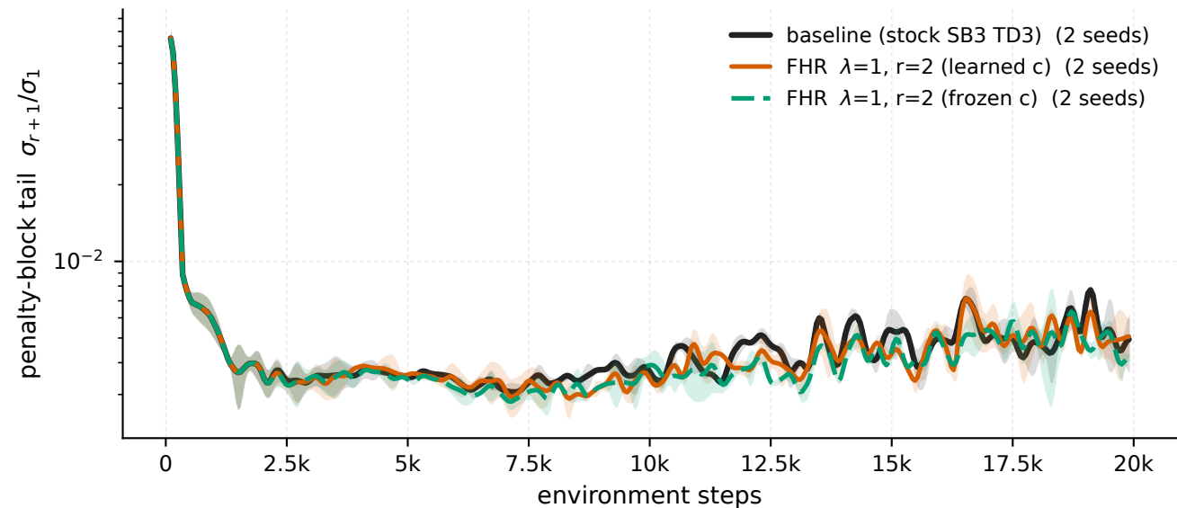
Pendulum-v1 - \lambda 1 \cdot r_2 , \lambda 1 \cdot r_2 frozen-c vs baseline, penalised windows penalty-block tail \sigma_{r+1}/\sigma_1
