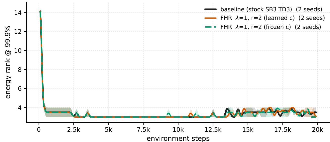
Pendulum-v1 - \lambda 1 \cdot r_2 , \lambda 1 \cdot r_2 frozen-c vs baseline, penalised windows energy rank @ 99.9%
