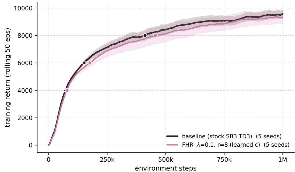
HalfCheetah-v5 - \lambda 0.1 \cdot r_8 vs baseline (training stream)
