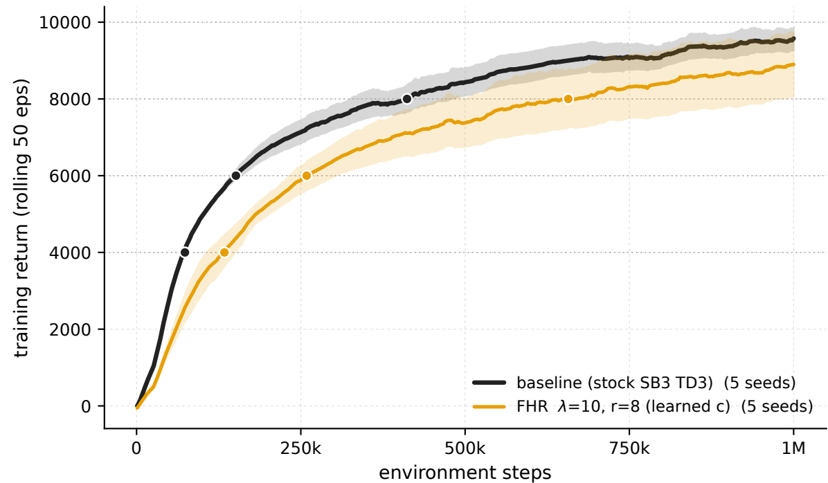
HalfCheetah-v5 - \lambda 10 \cdot r8 vs baseline (training stream)
