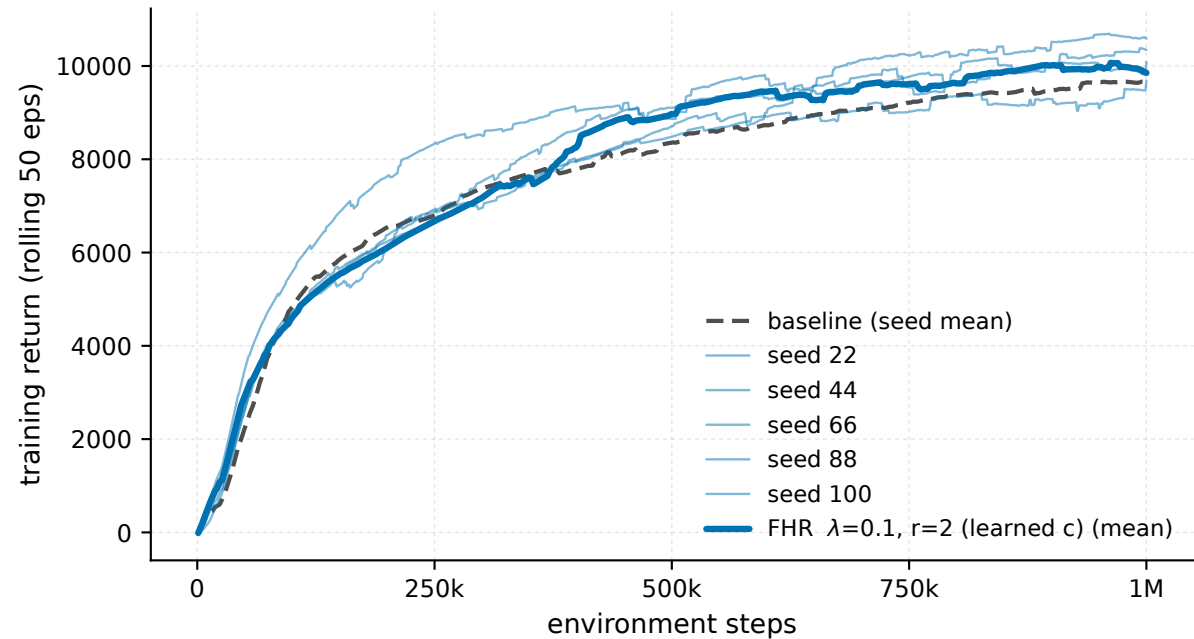
HalfCheetah-v5 - \lambda 0.1 \cdot r_2 , every seed (train)
