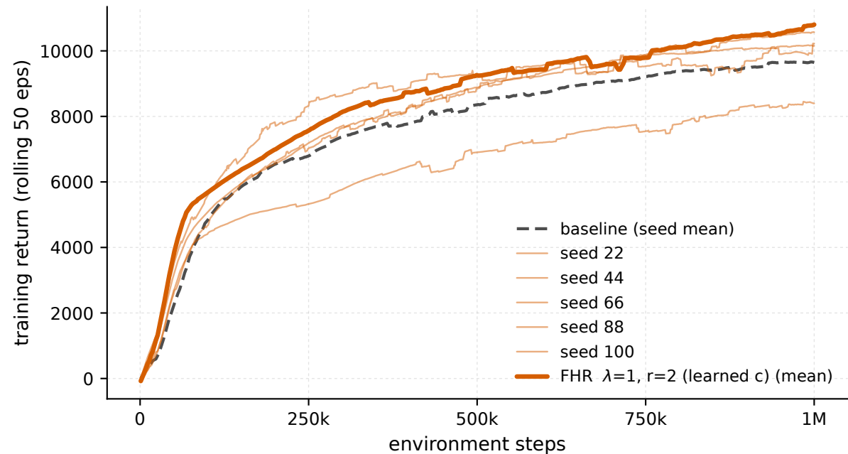
HalfCheetah-v5 - \lambda 1 \cdot r_2 , every seed (train)
