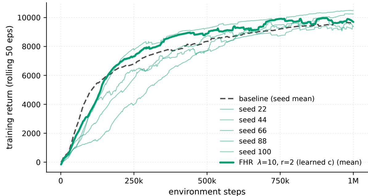
HalfCheetah-v5 - \lambda 10 \cdot r_2 , every seed (train)
