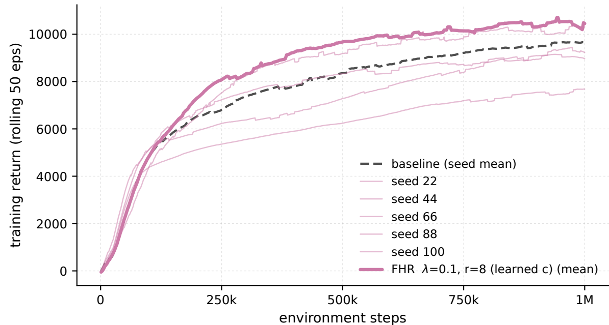
HalfCheetah-v5 - \lambda 0.1 \cdot r8 , every seed (train)
