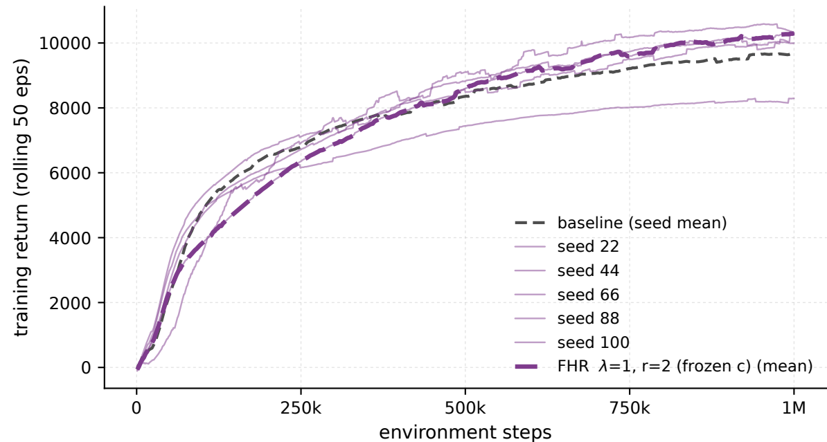
HalfCheetah-v5 - \lambda 1 \cdot r_2 frozen-c, every seed (train)
