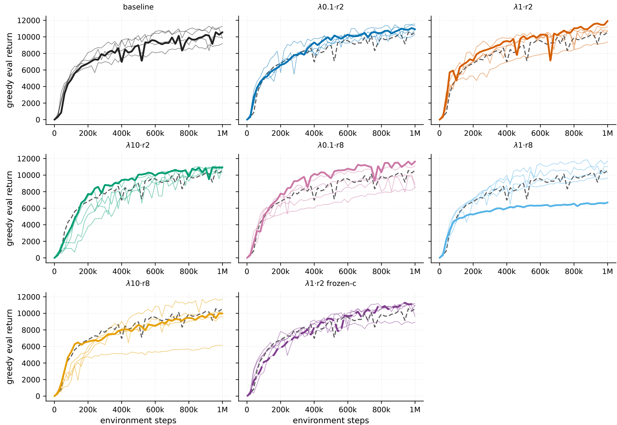
HalfCheetah-v5 - every seed per arm (eval); grey dashed = baseline seed mean
