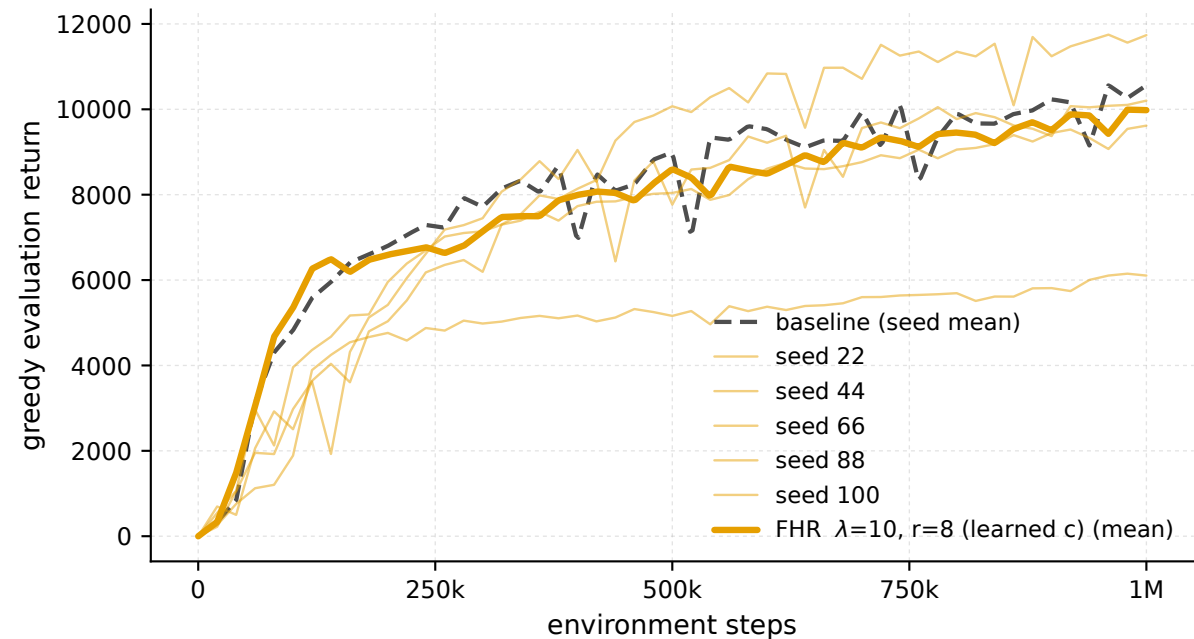
HalfCheetah-v5 - \lambda 10 \cdot r8 , every seed (eval)
