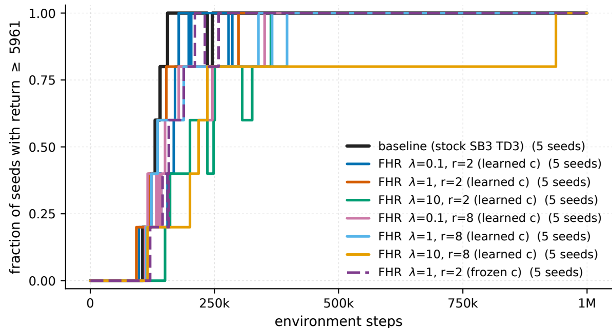
HalfCheetah-v5 - seeds above 5961 (eval)
