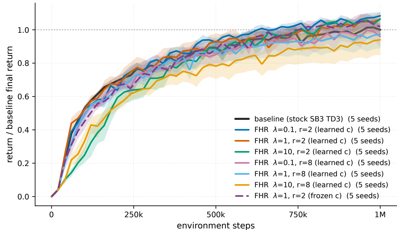
HalfCheetah-v5 - all arms, baseline-normalised (eval)
