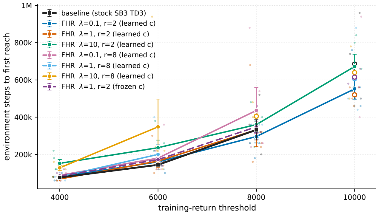
HalfCheetah-v5 - sample efficiency, greedy-eval stream (mean \pm 1 s.e.m.) open marker: not all seeds reached it
