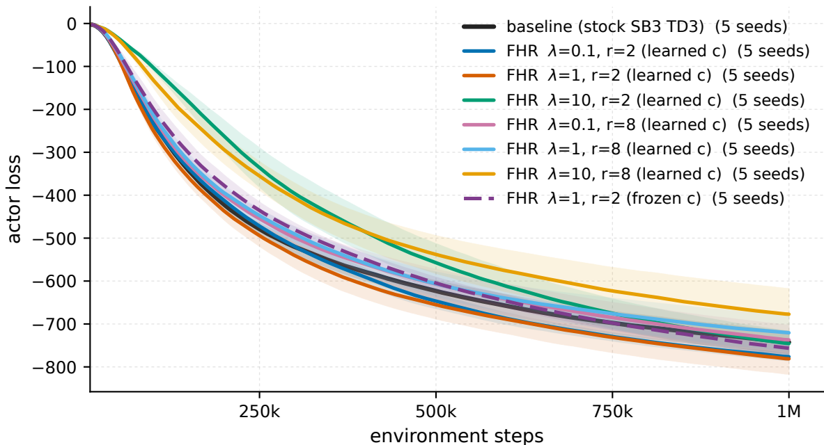
HalfCheetah-v5 - actor loss
