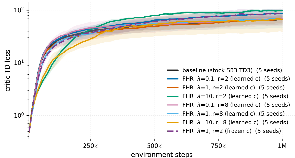
HalfCheetah-v5 - critic TD loss
