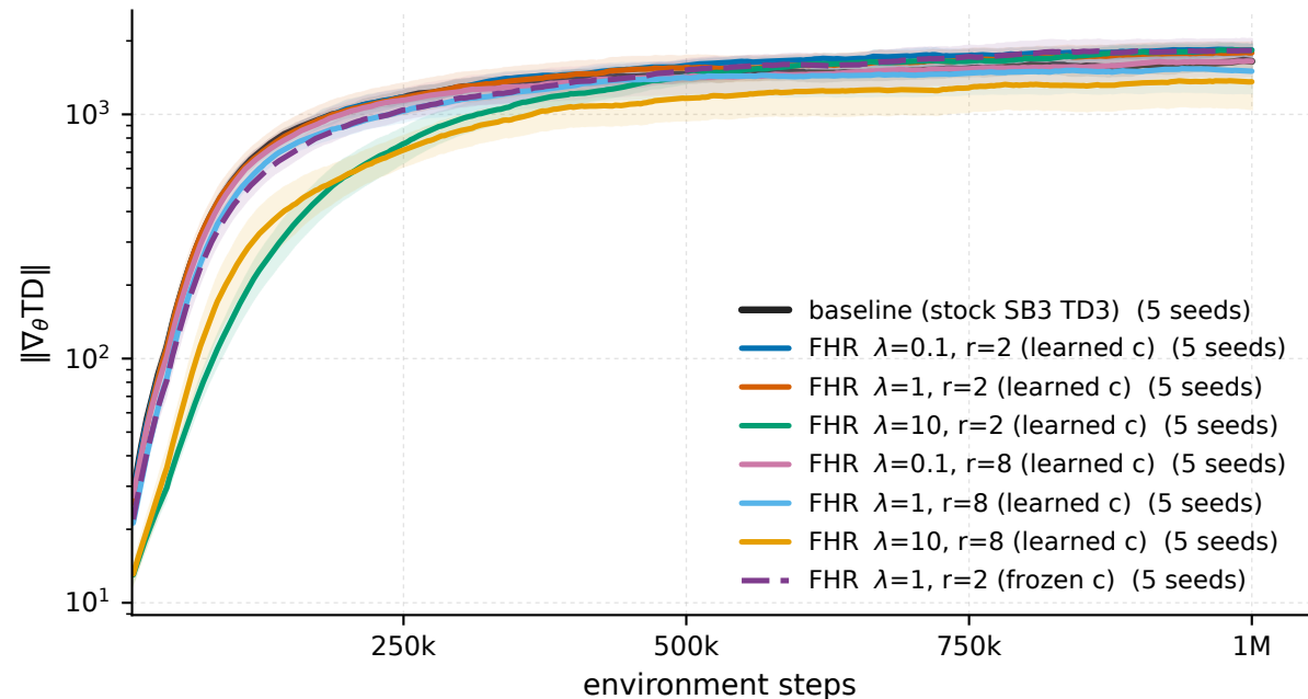
HalfCheetah-v5 - \|\nabla_{\theta}TD\|
