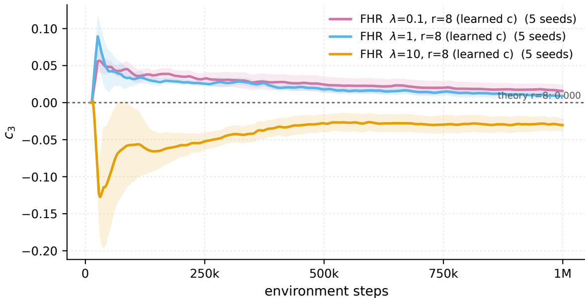
HalfCheetah-v5 - recurrence coefficient c_3 vs the Bellman theory value
