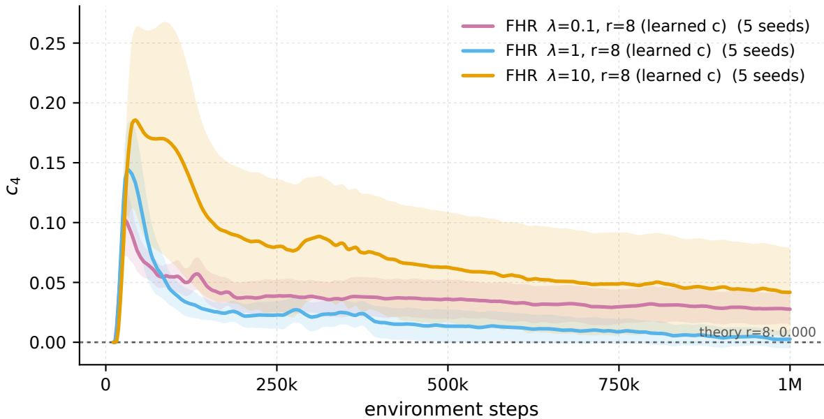
HalfCheetah-v5 - recurrence coefficient c_4 vs the Bellman theory value
