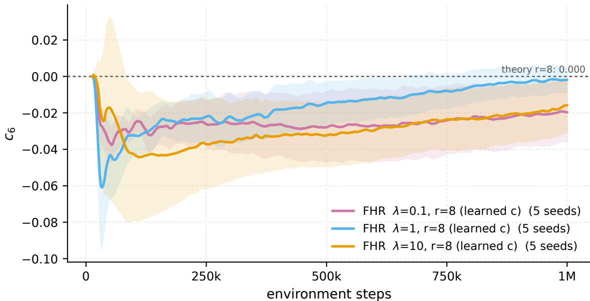
HalfCheetah-v5 - recurrence coefficient c_6 vs the Bellman theory value
