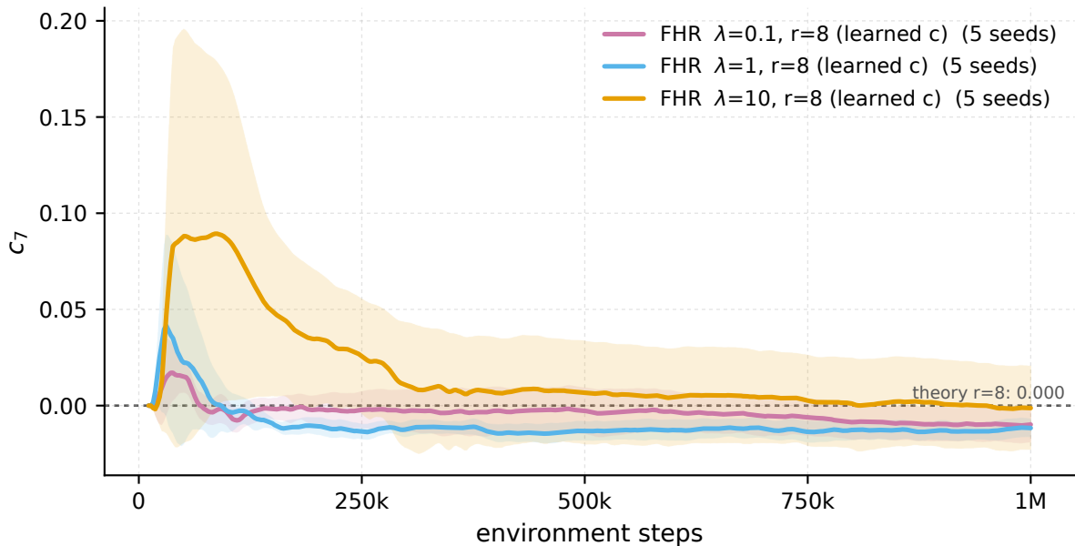
HalfCheetah-v5 - recurrence coefficient c_7 vs the Bellman theory value
