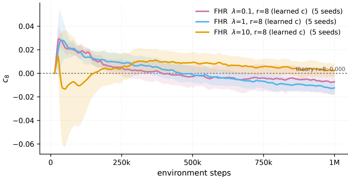
HalfCheetah-v5 - recurrence coefficient c_8 vs the Bellman theory value
