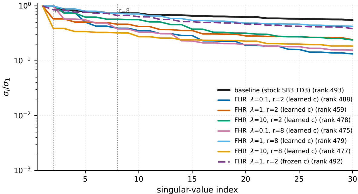
HalfCheetah-v5 - Hankel( \pi(s_t)_2 ) of the final policy (action dim 2)
