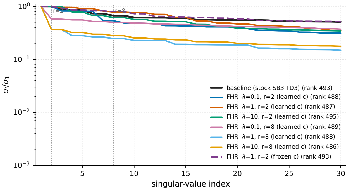
HalfCheetah-v5 - Hankel( \pi(s_t)_3 ) of the final policy (action dim 3)
