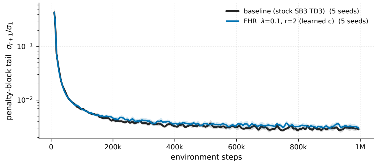
HalfCheetah-v5 - \lambda 0.1 \cdot r_2 vs baseline, penalised windows penalty-block tail \sigma_{r+1}/\sigma_1
