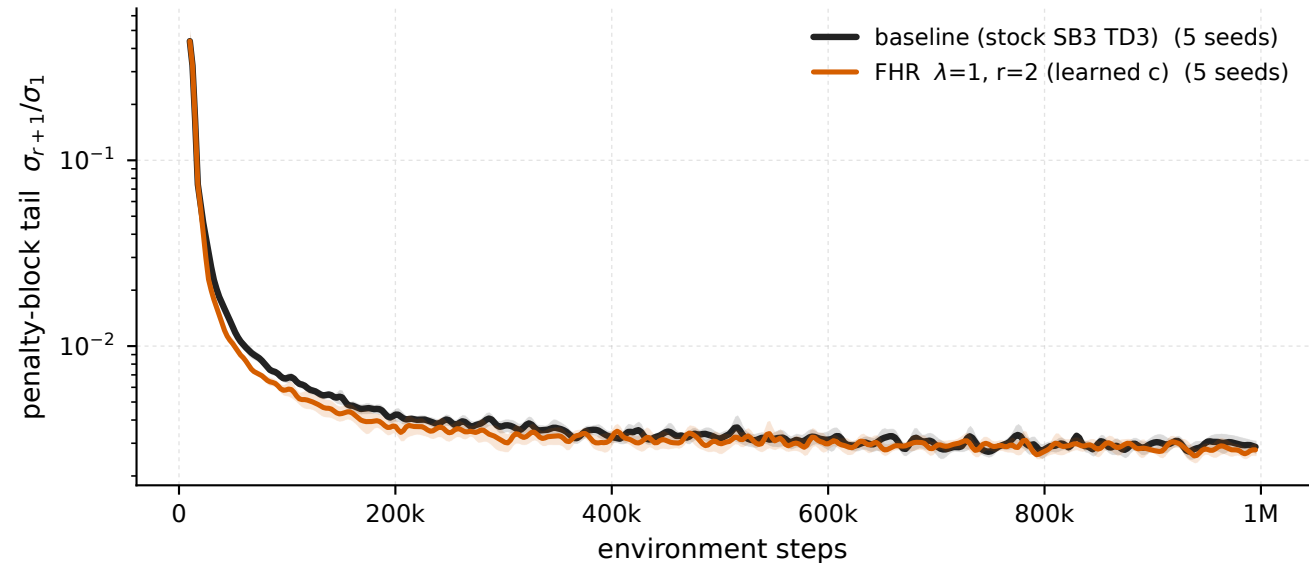
HalfCheetah-v5 - \lambda 1 \cdot r_2 vs baseline, penalised windows penalty-block tail \sigma_{r+1}/\sigma_1
