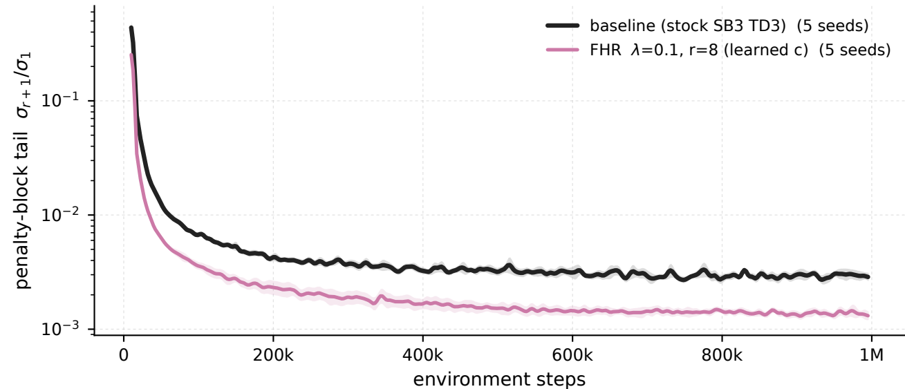
HalfCheetah-v5 - \lambda 0.1 \cdot r_8 vs baseline, penalised windows penalty-block tail \sigma_{r+1}/\sigma_1
