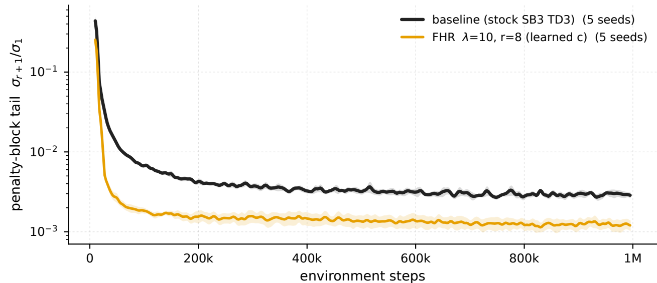
HalfCheetah-v5 - \lambda 10 \cdot r8 vs baseline, penalised windows penalty-block tail \sigma_{r+1}/\sigma_1
