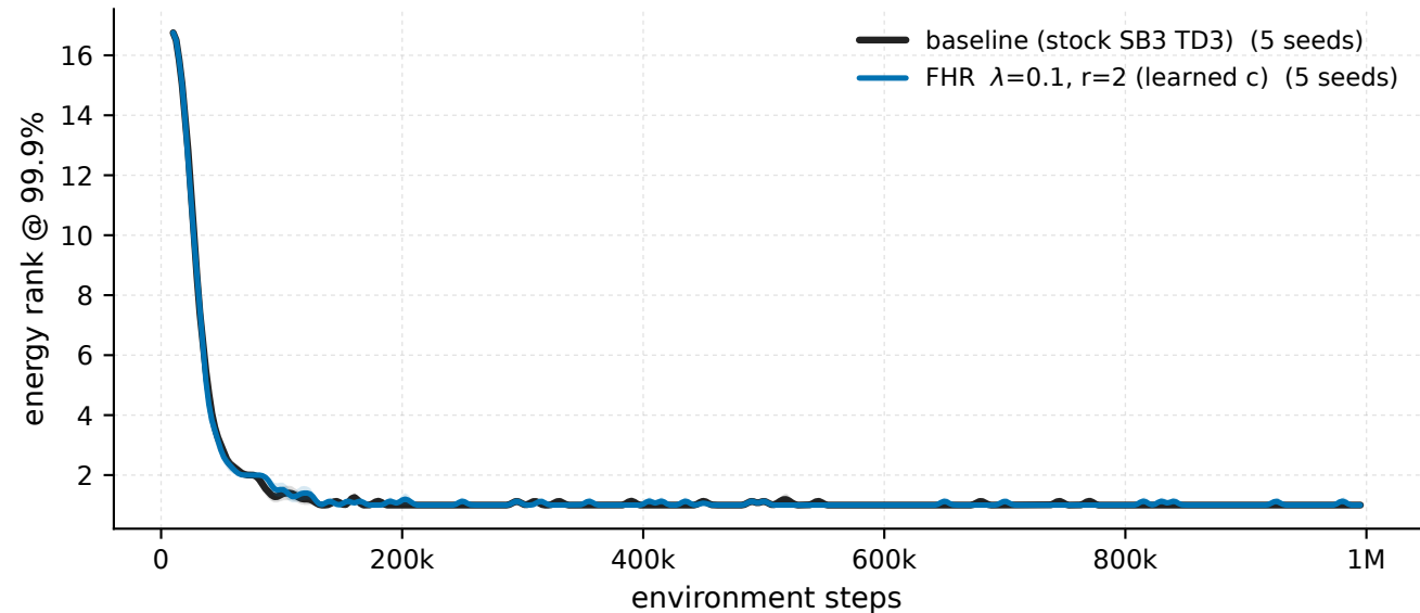
HalfCheetah-v5 - \lambda 0.1 \cdot r_2 vs baseline, penalised windows energy rank @ 99.9%
