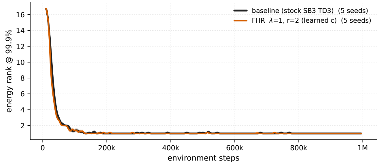
HalfCheetah-v5 - \lambda 1 \cdot r_2 vs baseline, penalised windows energy rank @ 99.9%
