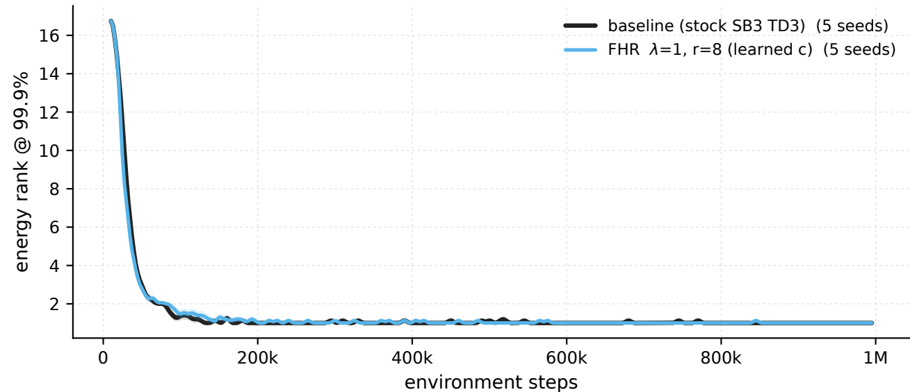
HalfCheetah-v5 - \lambda 1 \cdot r8 vs baseline, penalised windows energy rank @ 99.9%
