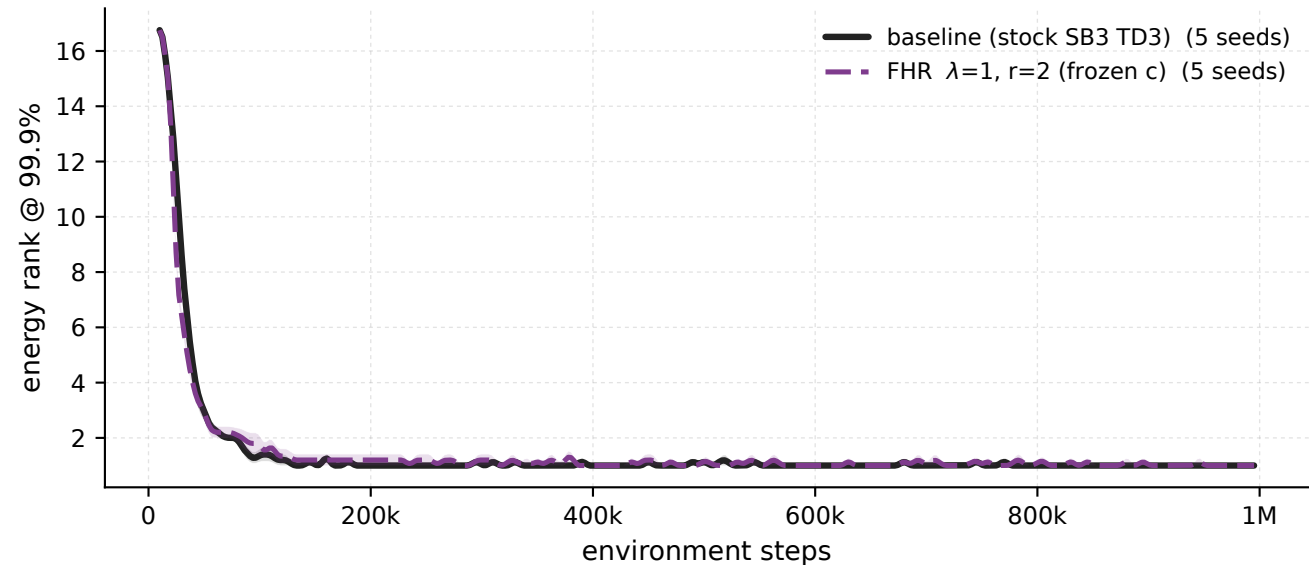
HalfCheetah-v5 - \lambda 1 \cdot r 2 frozen-c vs baseline, penalised windows energy rank @ 99.9%
