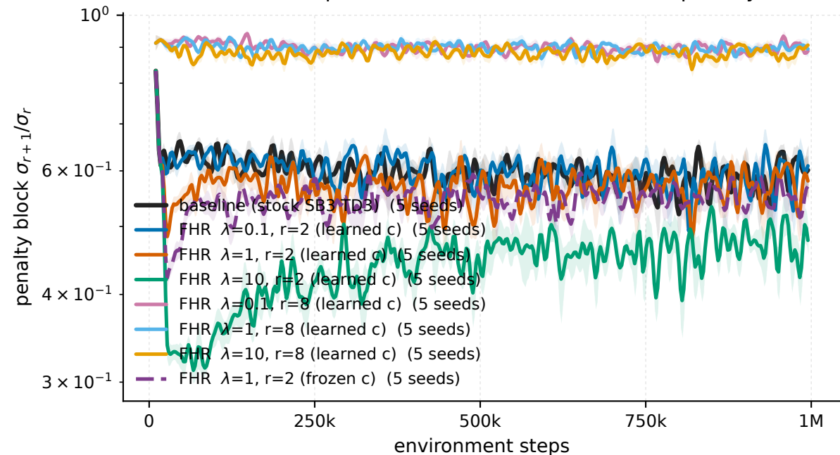
HalfCheetah-v5 - penalised windows: \sigma_{r+1}/\sigma_r of the penalty block
