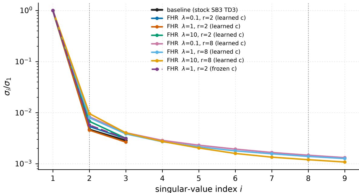
HalfCheetah-v5 - penalty block spectrum, final 25% of training (median over seeds and critics)
