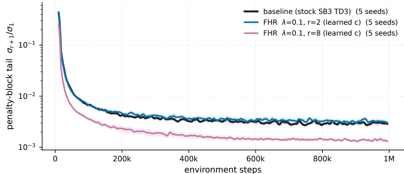
HalfCheetah-v5 - \lambda 0.1 \cdot r_2 , \lambda 0.1 \cdot r_8 vs baseline, penalised windows penalty-block tail \sigma_{r+1}/\sigma_1
