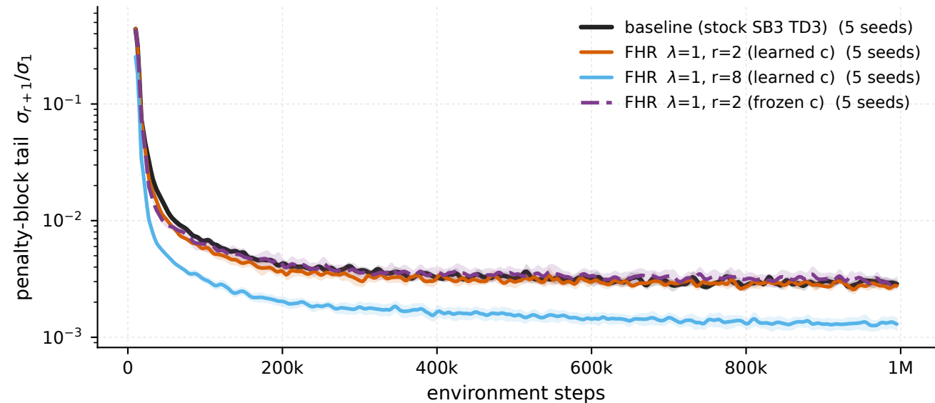
HalfCheetah-v5 - \lambda 1 \cdot r2 , \lambda 1 \cdot r8 , \lambda 1 \cdot r2 frozen-c vs baseline, penalised windows penalty-block tail \sigma_{r+1}/\sigma_1
