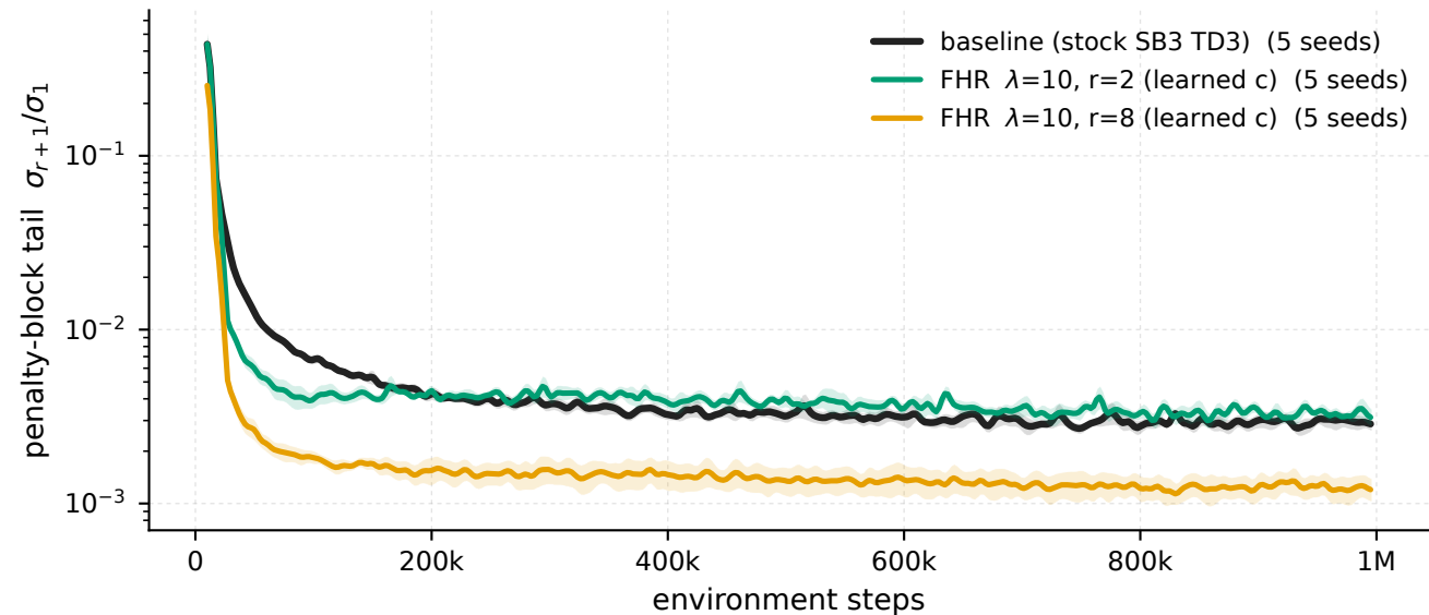
HalfCheetah-v5 - \lambda 10 \cdot r_2 , \lambda 10 \cdot r_8 vs baseline, penalised windows penalty-block tail \sigma_{r+1}/\sigma_1
