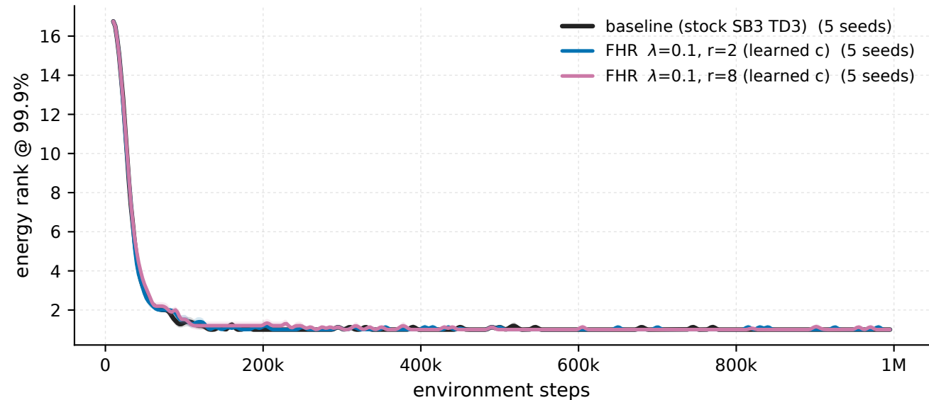
HalfCheetah-v5 - \lambda 0.1 \cdot r_2 , \lambda 0.1 \cdot r_8 vs baseline, penalised windows energy rank @ 99.9%
