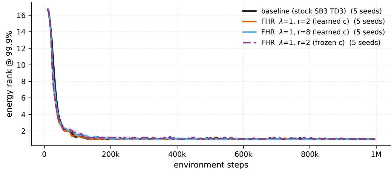
HalfCheetah-v5 - \lambda 1 \cdot r 2 , \lambda 1 \cdot r 8 , \lambda 1 \cdot r 2 frozen-c vs baseline, penalised windows energy rank @ 99.9%
