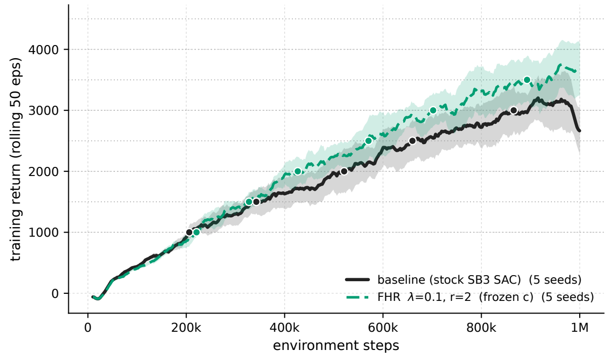
Ant-v5 - \lambda 0.1 \cdot r_2 frozen-c vs baseline (training stream)
