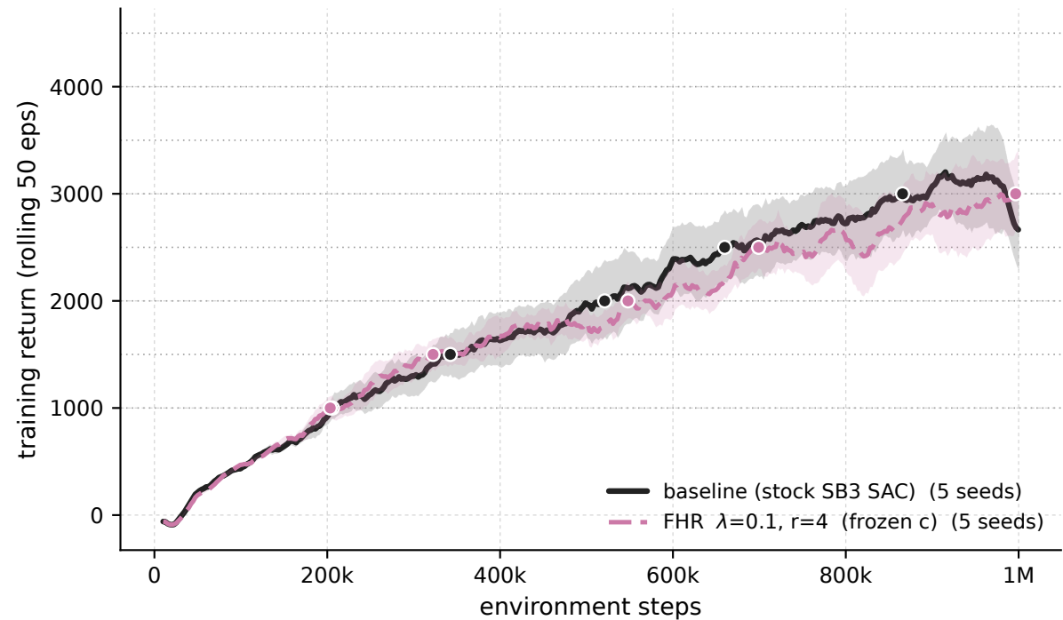
Ant-v5 - \lambda 0.1 \cdot r 4 frozen-c vs baseline (training stream)
