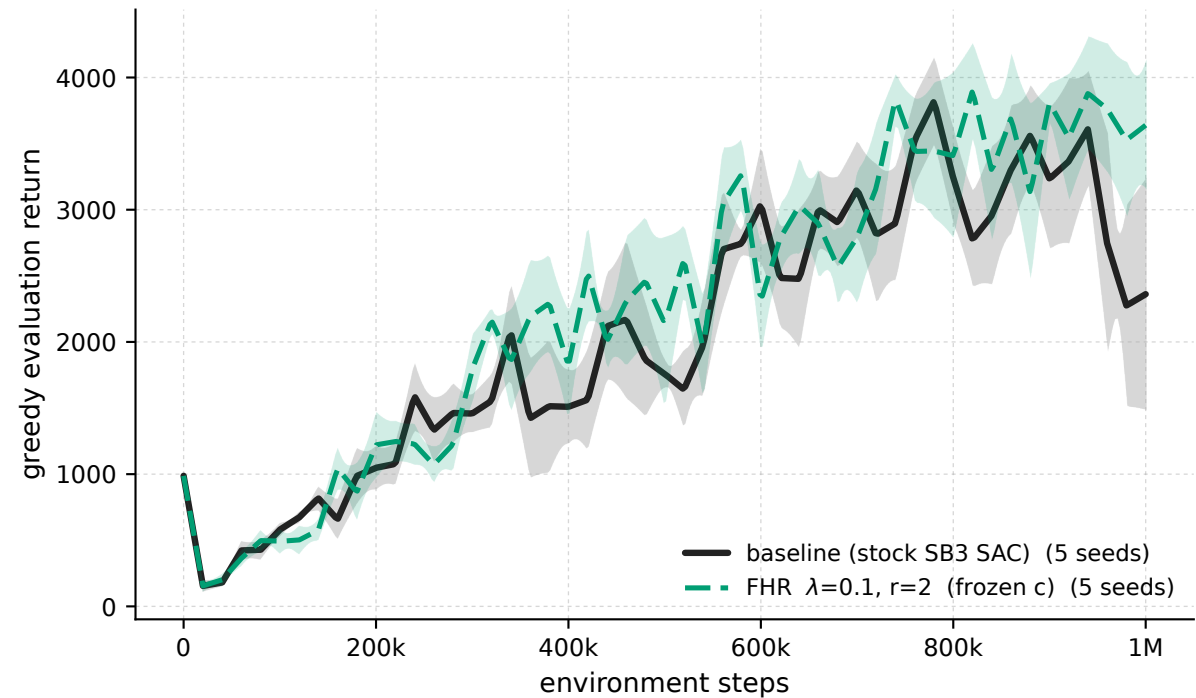
Ant-v5 - \lambda 0.1 ·r2 frozen-c vs baseline (greedy eval)
