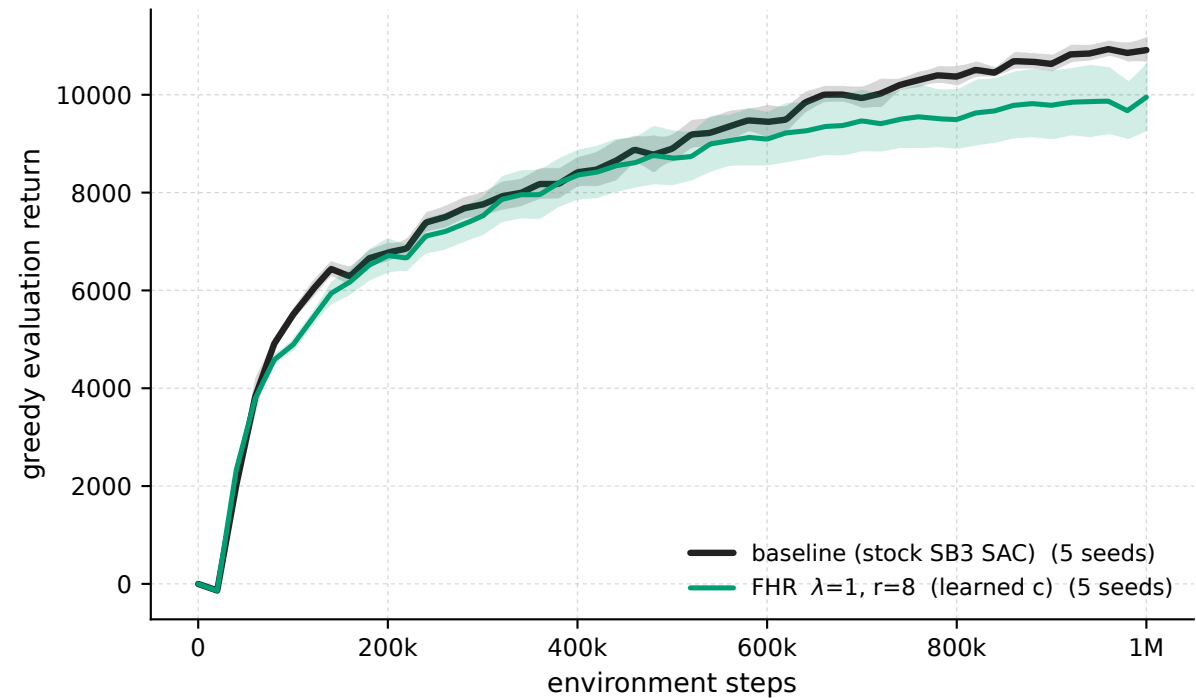
HalfCheetah-v5 - \lambda 1 \cdot r 8 vs baseline (greedy eval)
