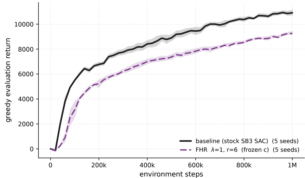
HalfCheetah-v5 - \lambda=1 , r=6 frozen-c vs baseline (greedy eval)
