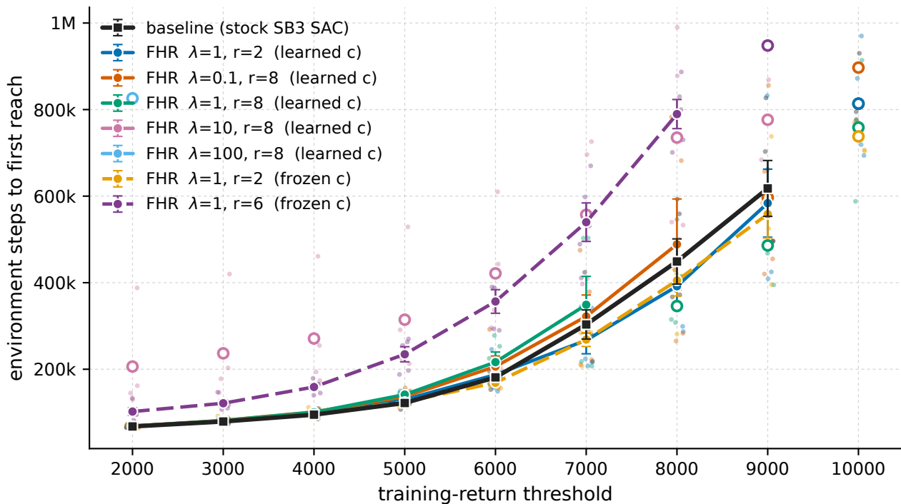
HalfCheetah-v5 - sample efficiency, training stream (mean \pm 1 s.e.m.) open marker: not all seeds reached it
