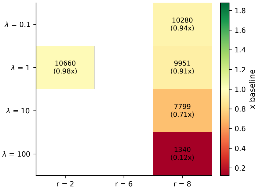
final return vs baseline (10913)
