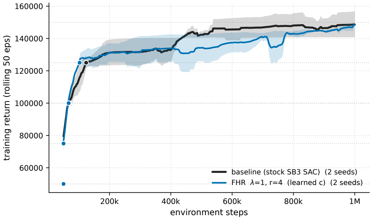
HumanoidStandup-v5 - \lambda 1 \cdot r4 vs baseline (training stream)
